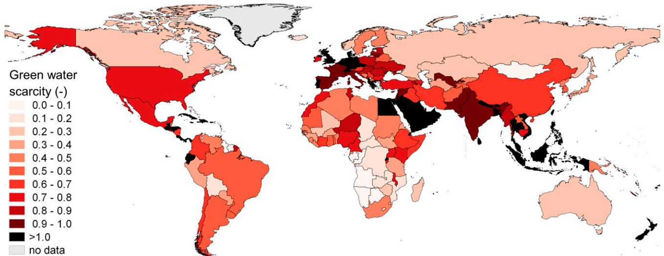
Fig. 3. WS g per country, expressed as the ratio of the national aggregate WF g to the national aggregate WF g,m . Countries with WS g = 1 have fully allocated their sustainably available green water flow to human activities (or overshoot is canceled out by remaining potential in another part of the country). Country-specific estimates of WF g , WF g,m , WS g , and overshoot as percentage of WF g are included in SI Appendix, Table S1 .
